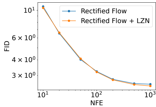
Figure 24: FID vs. number of sampling steps in the Euler sampler on CIFAR10 (conditional generation). RF+LZN outperforms RF in most cases.
