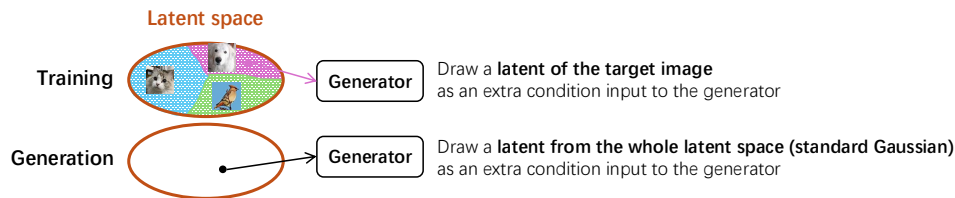
Figure 4: LZN for unconditional generative modeling (§ 3). During training, the LZN latent of each target image is fed as an extra condition to the rectified flow (RF) model [53], making the RF learn conditional flows based on LZN latents. The objective remains the standard RF loss, and the LZN encoder is trained end-to-end within it. During generation, we sample LZN latents from a standard Gaussian and use them as the extra condition. We illustrate the approach with RF, but since LZN latents require no supervision and are differentiable, the method could apply to other tasks by adding a condition input for LZN latents to the task network.
