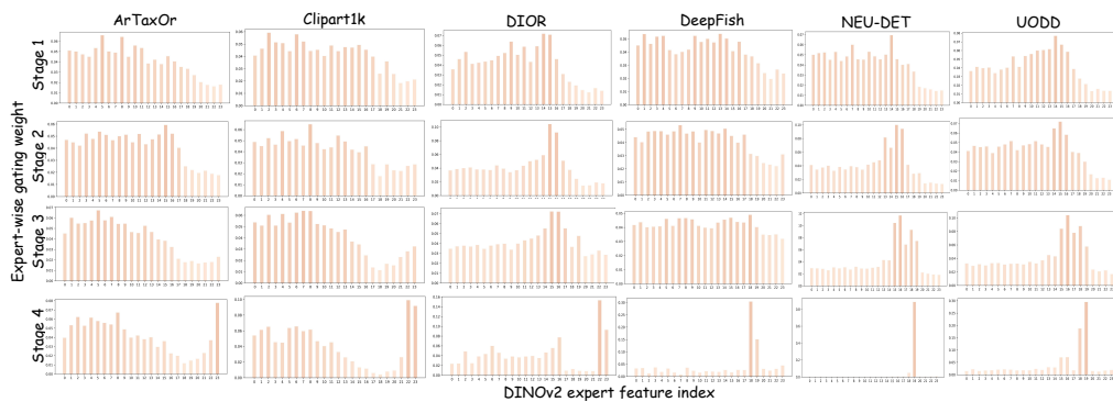
Figure 5: Expert feature selection at different layers of the backbone. The horizontal axis represents expert features, the vertical axis represents the expert-wise gating weights at different layers.
