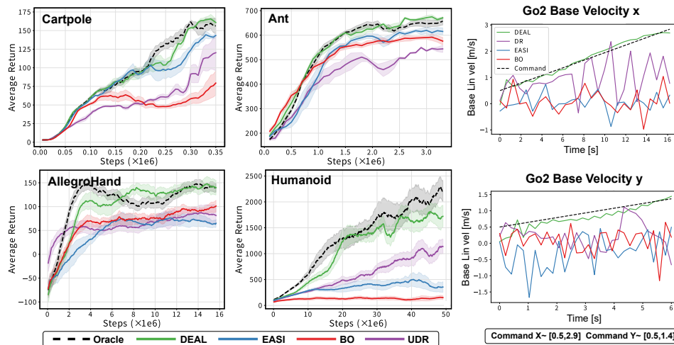
Figure 4: Left: The average return in the target environment for the policies trained at each stage with DEAL and other sim-to-real baselines. Right: The speed tracking display of Go2 under training with DEAL and other sim-to-real baselines. up: speed in the robot's x-axis direction, down: speed in the robot's y-axis direction.
