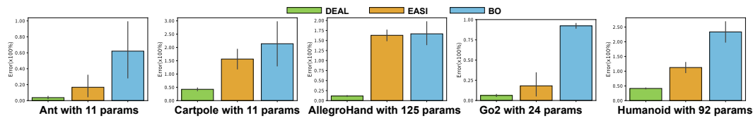
Figure 3: Average search errors for each method, consisting of the error percentage of all parameters.
