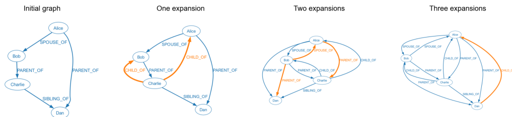
Figure 5: A toy example of iterative graph expansion. From left to right: The initial family tree graph is shown. When the graph autoencoder model for link prediction is applied to this graph, the links shown in orange, which have a probability greater than 0.5, are added. The graph autoencoder is then applied to this expanded graph.
