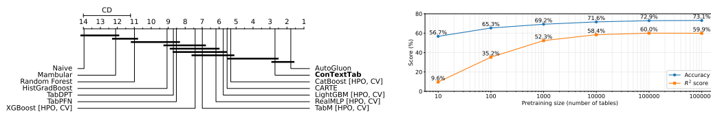
Figure 2: Left: critical difference diagram between ConTextTab and several baselines, across the CARTE benchmark. Right: Impact of pretraining dataset size on validation accuracy and R^2 scores.
