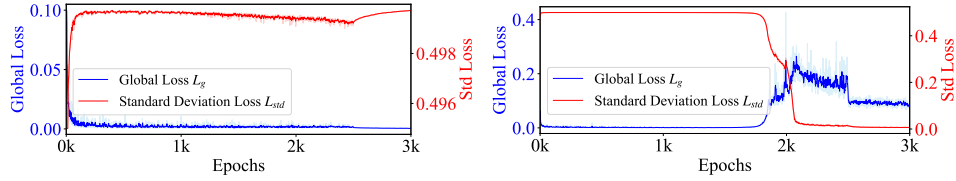
Figure 3: Comparison of global and standard deviation loss on validation data between the same two runs learning on only zero Chern numbers, as shown in Figure 4. The former, without TrNorm layers, collapses to zero local quantities everywhere, hence having a lower L_g on trivial samples, yet could not generalize to nontrivial cases. In contrast, the latter, with TrNorm layers, succeeds in learning global quantities and local differences simultaneously.
