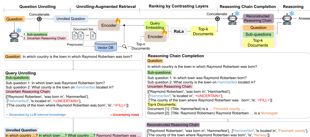
Figure 1: Overview of CoopRAG, which consists of: (i) Question Unrolling, (ii) Unrolling-Augmented Retrieval, (iii) Ranking by Contrasting Layers (RaLa), (iv) Reasoning Chain Completion, and (v) Reasoning
