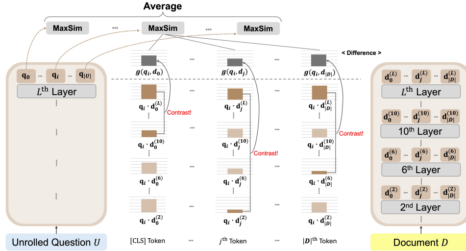
Figure 2: Illustration of the Ranking by Contrasting Layers (RaLa) process before optimization, corresponding to Equation 3.
