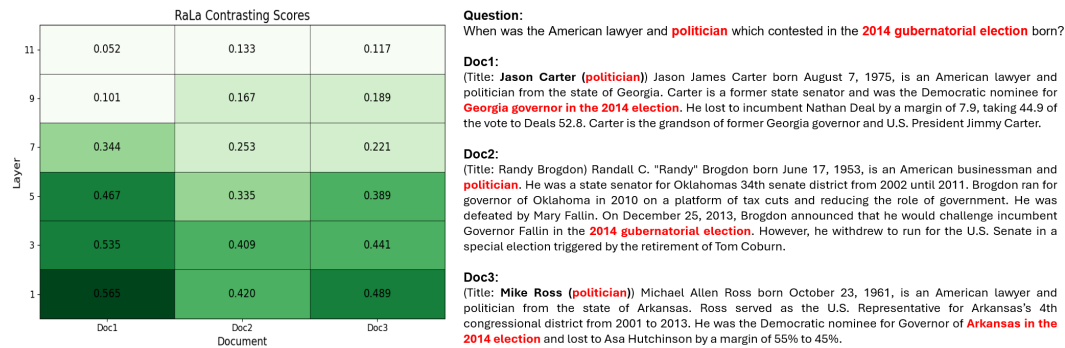
Figure 8: Illustrative example of RaLa. For each document, the heatmap displays the scores obtained by applying RaLa between the final, i.e., 12th, layer and premature odd-numbered layers (1, 3, 5, 7, 9, 11). An input question, a ground-truth document, and two negative documents are described to the right.
