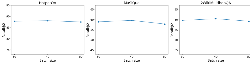
Figure 6: Hyperparameter sensitivity analysis on batch size, showing Recall@2 for batch sizes of 30, 40, and 50 across datasets (HotpotQA, MuSiQue, and 2WikiMultihopQA).
