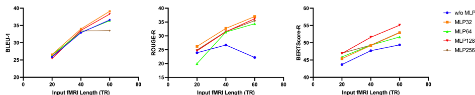
Figure 5: Parameter settings for dimensionality of the MLP in semantic wrap-up.
