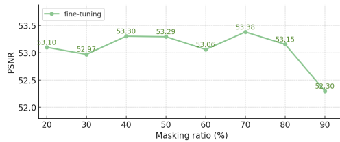
(a) Effect of masking ratio during MVM-LF pretraining.
