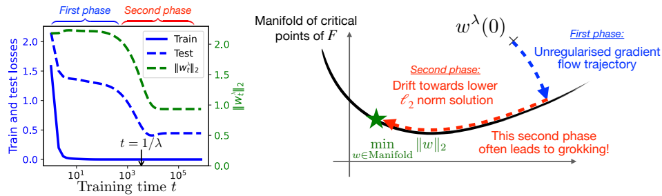
Figure 1: Gradient flow with small weight decay \lambda . (Left) A typical example of grokking: the training loss rapidly drops to zero, while the test loss plateaus for a long period before eventually decreasing—coinciding with a steady drop in the \ell_2 -norm of the weights. (Right) Schematic illustration in parameter space \mathbb{R}^d of the optimisation behaviour described in Theorem 1. The trajectory w^\lambda(t) initially follows the unregularised gradient flow and converges to a manifold of critical points of F (fast dynamics). At time t \approx 1/\lambda , the regularisation term becomes dominant and induces a slow drift along this manifold toward a lower \ell_2 -norm solution (slow dynamics).
