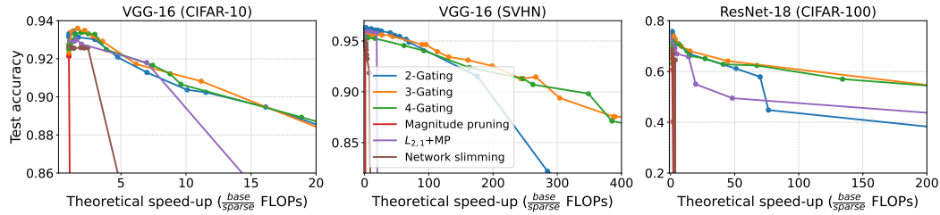
Figure 11: Test accuracy vs. theoretical speed-up (measured as the ratio of FLOPs) of D -Gated convolutional neural networks and comparison methods.
