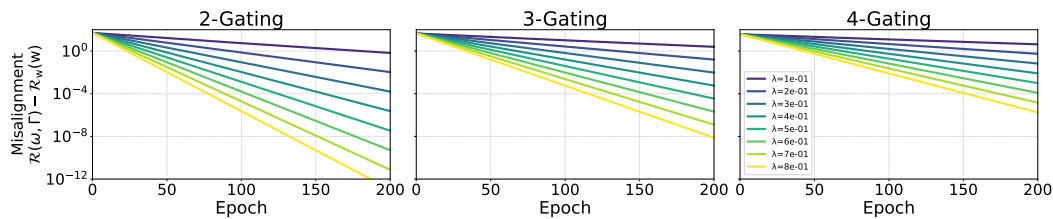
Figure 17: Convergence of regularizers, i.e., evolution of misalignment, instead of loss convergence for SGD trained on a neuron-sparse LeNet-300-100. Setting is the same as for Fig. 3.
