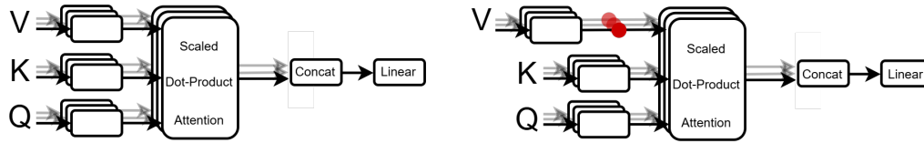
Figure 9: Schematic illustration of D -Gating overparameterization to achieve structured head sparsity in a multi-head attention layer. Left: original attention layer. Right: D -Gated value matrices sparsify the whole attention head. Red nodes indicate the location of the additional gating parameters.
