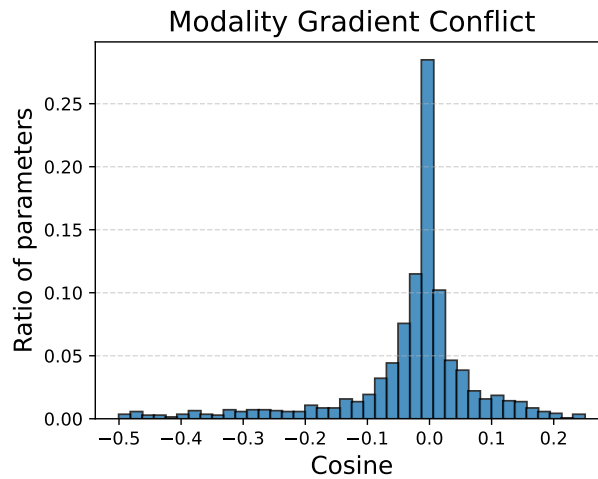
Figure 5: Cosine distance distribution between text and image modality gradients in modality-coupled MoE LoRA [44] on the ScienceQA [58] dataset. The y-axis shows the proportion of parameters corresponding to each cosine distance. Lower cosine distance values indicate greater gradient conflict, with 0 denoting orthogonal update directions.
