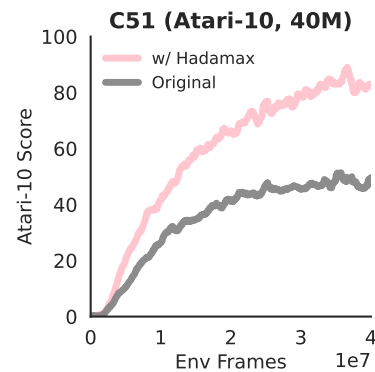
Figure 7: C51 with and without a Hadamax encoder on Atari-10.
