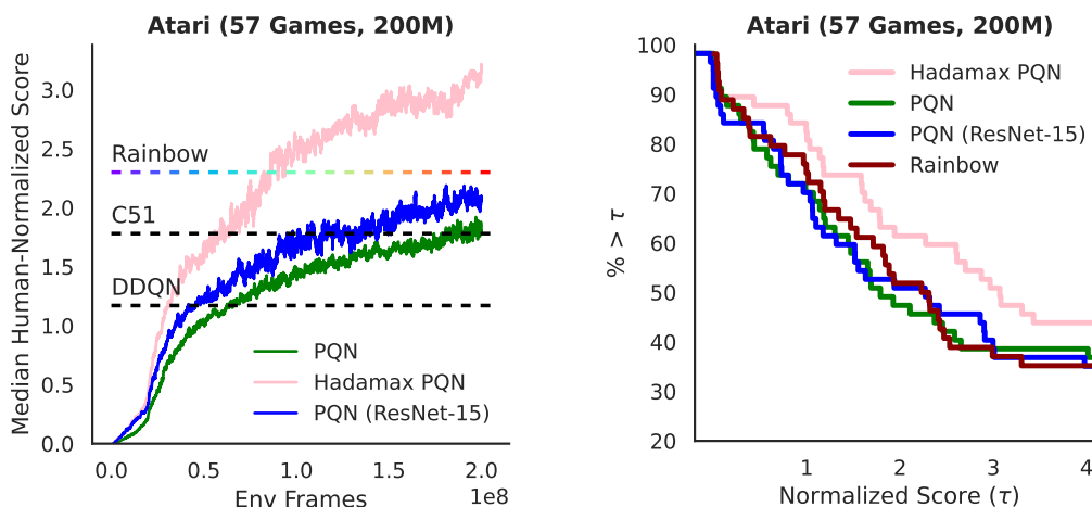
Figure 5: Median Human-Normalized performance training PQN, PQN (Resnet-15) and Hadamax-PQN in the Atari domain over 57 games, 200M frames and 5 seeds (left), and the Atari-57 score profile (right). The Atari-57 score profile illustrates the percentage of games that exceed the normalized score threshold on the x-axis.
