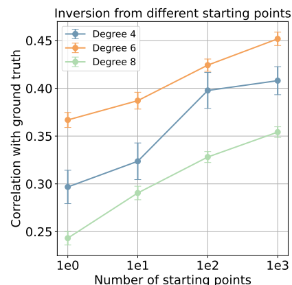
Figure 5: Inversion with increasing starting points. Correlation between the inverted models and the ground truth strengthens as the number of starting points increases. Performance on different degrees shows a consistent trend.
