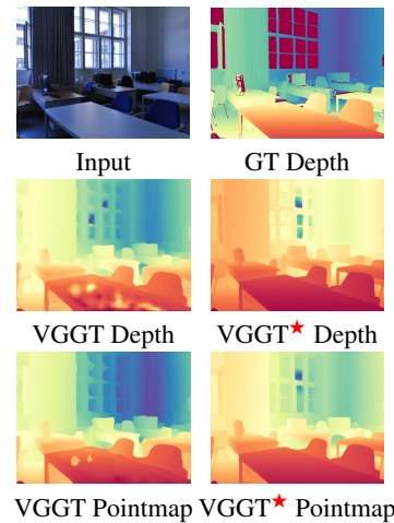
Figure 7: Depth from depth head and pointmap head of VGGT. ★ denotes our fine-tuning model.
