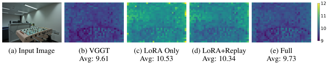
Figure 3: Heatmaps show spatial variations in L_2 norms of encoder patch tokens across configurations. “Avg” is the average norm of the feature map, and (e) Full indicates the full model with re-normalization LoRA and multi-view data replay.
