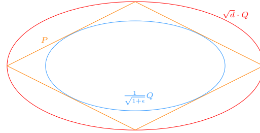
Figure 2: The geometric interpretation of the output ellipsoid. Let P be a given input polytope. We can find an ellipsoid Q so that \frac{1}{\sqrt{1+\epsilon}}Q \subseteq P \subseteq \sqrt{d} \cdot Q .
