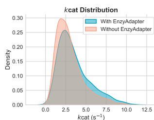
Figure 5: Comparison of k_{cat} distribution.
