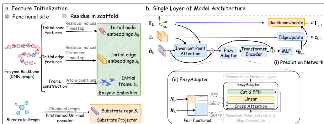
Figure 3: EnzyControl is a flexible approach for the conditional backbone generation of enzymes. (a) Feature Initialization involves obtaining initial node embeddings and edge embeddings, constructing initial frames for enzyme backbones, and initializing pretrained features for substrates. (b) Single-layer structure prediction network with EnzyAdapter.
