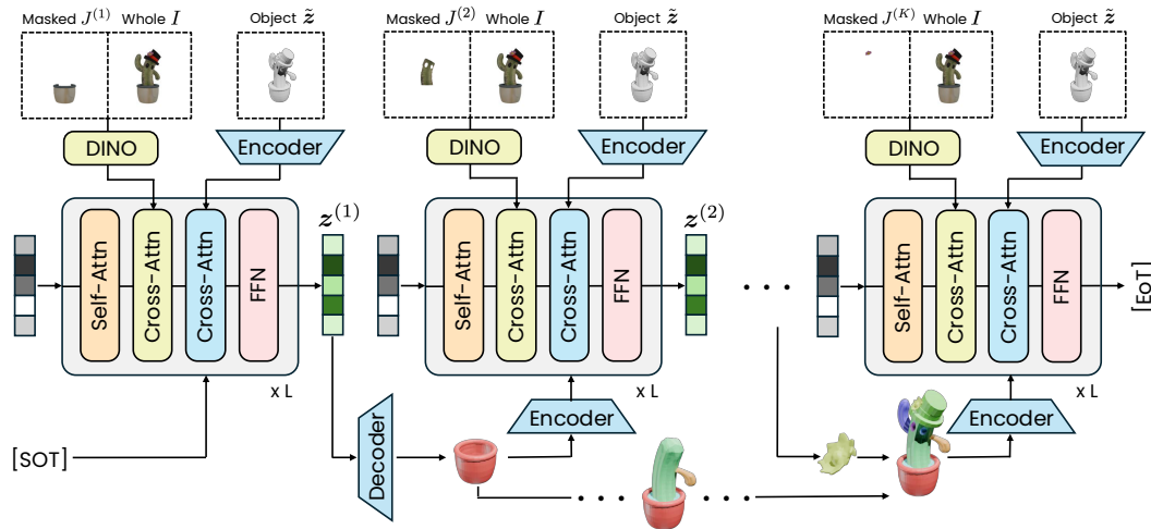
Figure 2: AutoPartGen generates parts autoregressively. At each step, a 3D latent diffusion model generate the next part, conditioned on the previously generated parts z^{(1,\dots,k)} , the overall object \tilde{z} , and, optionally, an image I of the object and an image J^{(k)} of the part. The latent representation uses 3DShape2VecSet and the diffusion model is a DiT.
