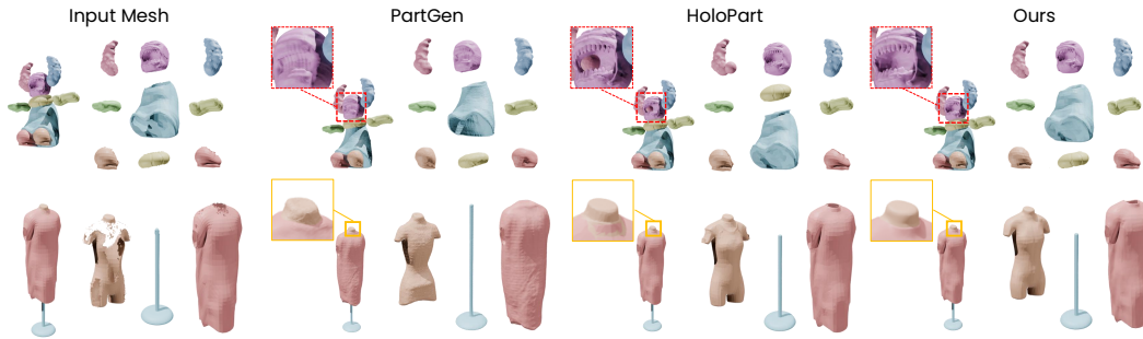
Figure 7: Visual comparison of different completion methods. Our approach achieves better geometric coherence by considering previously generated parts in context.
