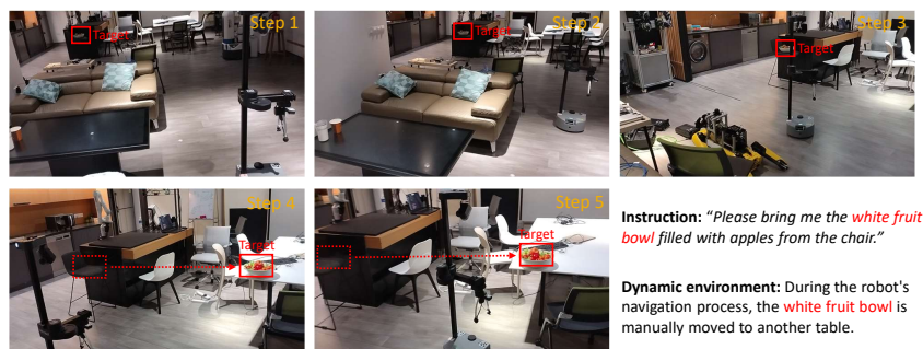
Figure 4: A demonstration of navigation in a dynamic real-world environment.
