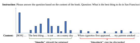
Figure 1: Visualization of attention scores from a single attention head during inference on the “Needle-in-a-Haystack” long-text benchmark. This benchmark requires the LLM to follow instructions and retrieve “needles” – specific pieces of information randomly inserted into a long text – to answer a given question. The evaluator heads are identified as those that accurately locate the relevant facts, thereby achieving high scores.
