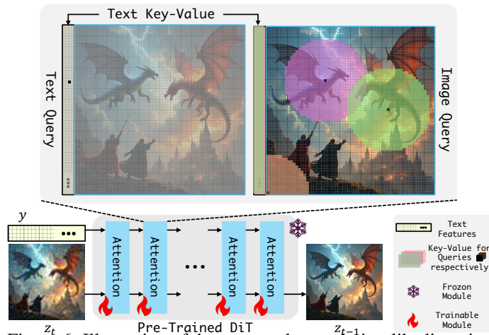
Figure 6: Illustration of the proposed convolution-like linearization strategy for pre-trained DiTs. In each text-image joint self-attention module, text queries aggregate information from all text and image tokens, while each image token gathers information only from tokens within a local circular window.
