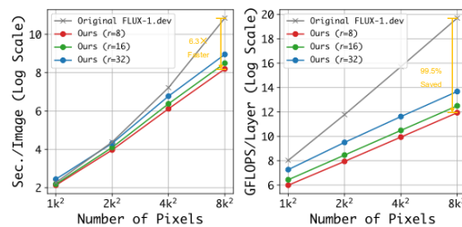
Figure 2: Comparison of speed and GFLOPS between the proposed linearized DiT and the original FLUX.1-dev. Speed is evaluated by performing 20 denoising steps on a single H100 GPU. FLOPS is calculated with the approximation: 4 \times \sum M \times c , where c is the feature dimension and M denotes the attention masks. \log_2 is applied on both vertical axes for better visualization. The raw data are supplemented in the appendix.
