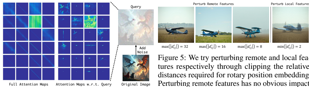
Figure 4: Visualization of attention maps by various heads. Attention in pre-trained DiTs is largely conducted in a local fashion.
