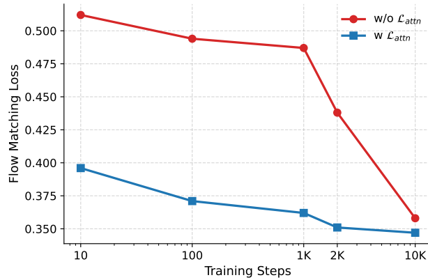
Figure 14: Effectiveness of \mathcal{L}_{attn} on accelerating the training convergence.
