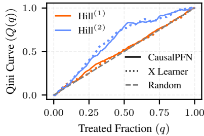
Figure 6: Hill (1) & Hill (2) Qini curves.
