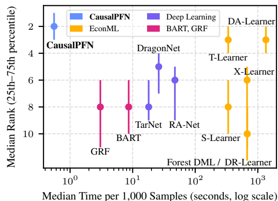
Figure 1: Time vs. Performance. Comparison across 310 causal inference tasks from IHDP, ACIC, and Lalonde. CausalPFN achieves the best average rank (by precision in estimation of heterogeneous effect) while being much faster than other baselines.
