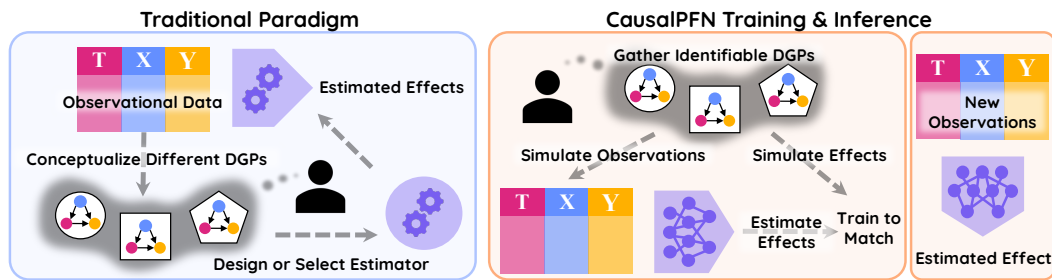
Figure 2: Traditional Causal Inference vs. CausalPFN. (Left): A domain expert manually builds or selects an estimator for a DGP that they deem appropriate for the given data. (Right): The domain expert simulates diverse DGPs for pre-training, and a transformer learns to amortize causal inference automatically.
