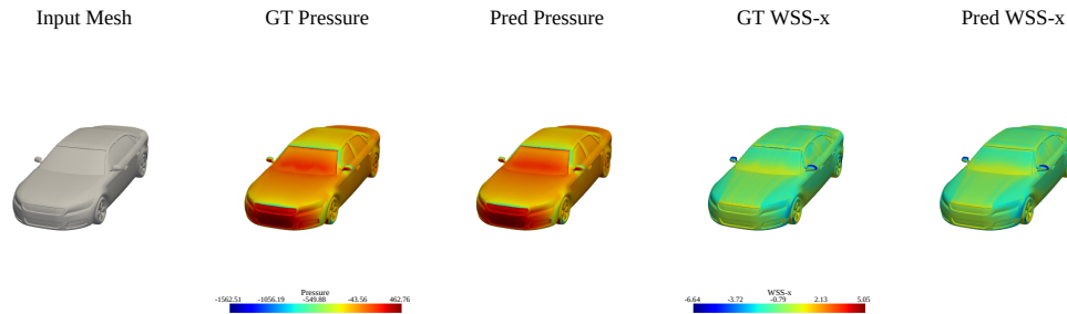
Figure 4: Comparison of predicted and ground-truth (GT) results for the pressure and wall shear stress in the x-direction (WSS-x) on the DrivAerNet++ test sample N_S_WWS_WM_172.
