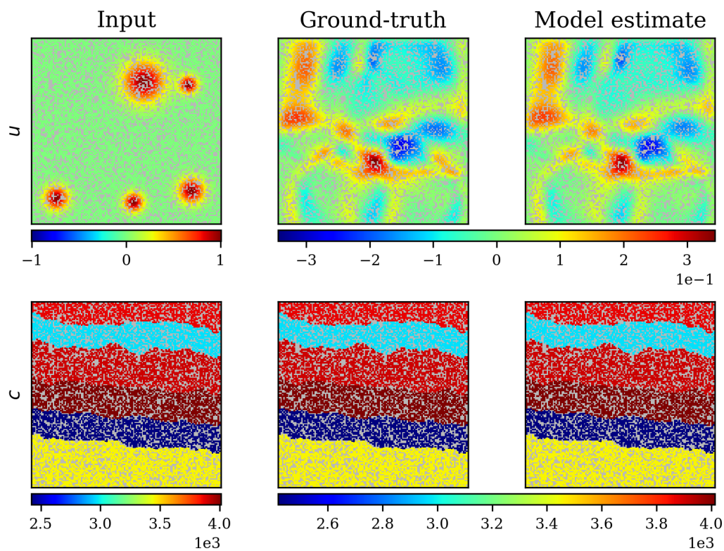
Figure G.20: Model input at t = t_0 , ground-truth solution and model estimate at t = t_{14} of a test sample unstructured Wave-Layer dataset.
