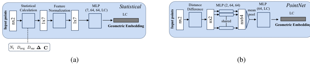
Figure B.2: Schematic of the Geometric Embedding for Statistical Embedding (a) and PointNet-based Embedding (b). LC denotes the lifting channels for MAGNO output.
