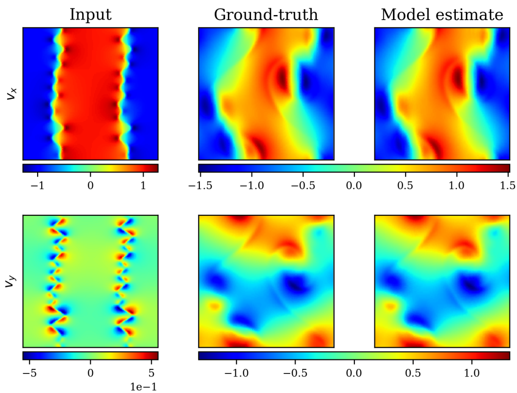
Figure G.24: Model input at t = t_0 , ground-truth solution and model estimate at t = t_{14} of a test sample NS-SL dataset.
