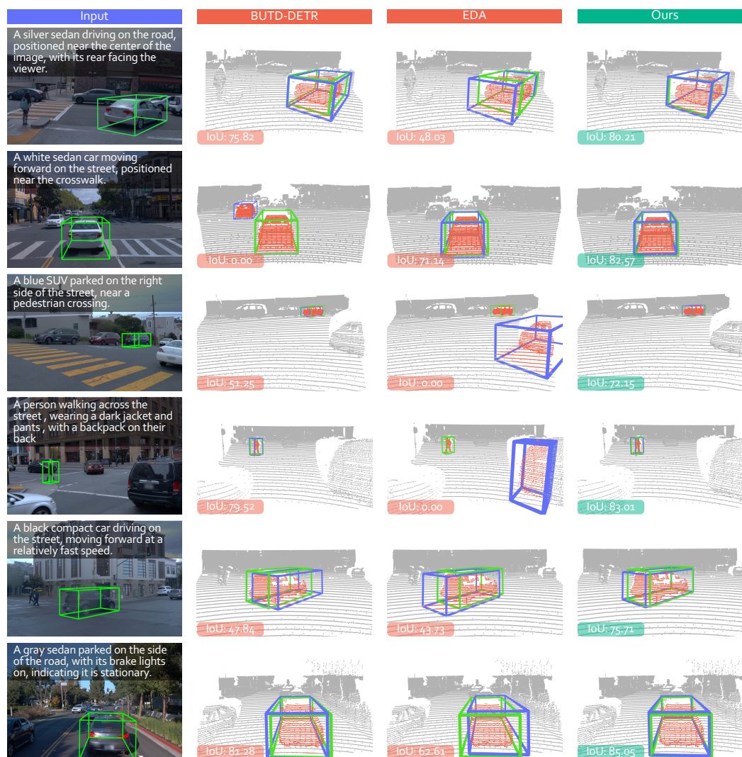
Figure 14: Additional qualitative comparisons of single-object 3D grounding on the Vehicle platform from the 3CED dataset. The data shown include the RGB frames, the LiDAR point clouds, and the associated referring expressions. The ground truth and predicted boxes are shown in green and blue, respectively. Best viewed in colors and zoomed in for more details.
