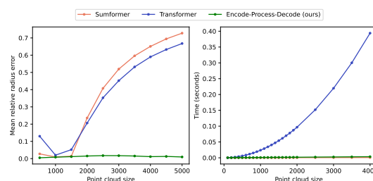
Figure 2: Comparison of error (left) and inference time (right) of the Transformer, Sumformer, and encode-process-decode approaches for estimating the radius of the minimum enclosing ball.
