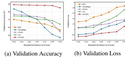
Figure 3: D-GDA encourages flatter minima.
