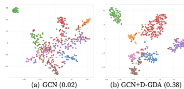
Figure 4: t-SNE of node embeddings on Cora.
