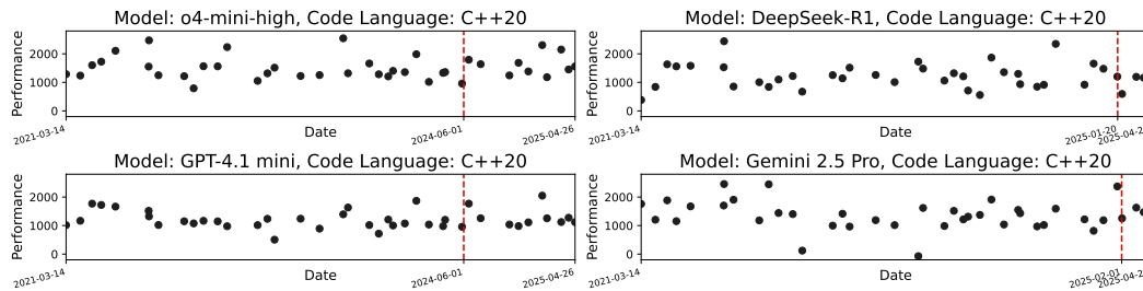
Figure 6: Investigation of contamination. For each model, a scatter plot is shown with contest end dates on the x-axis and performance on the y-axis. The red vertical line indicates the knowledge cutoff date of the model. For DeepSeek-R1, its release date was used as official information is unavailable.
