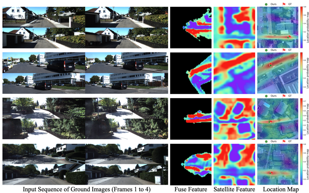
Figure 7: Visualization of multi-frame localization results on the KITTI dataset, achieved using our BevSplat-based approach. This demonstrates the aggregation of information over time and the filtering of dynamic elements.
