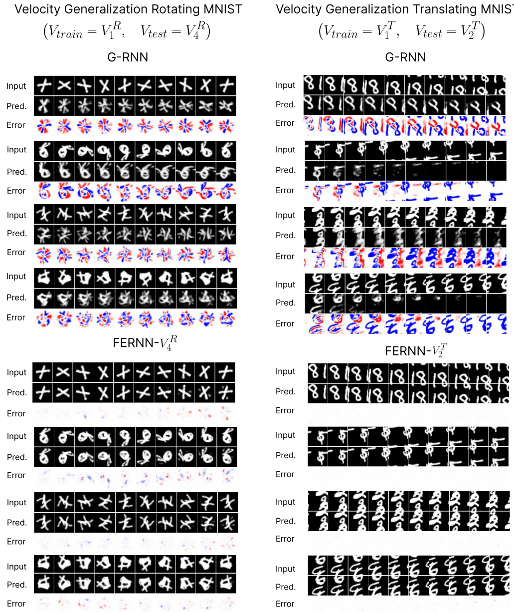
Figure 15: Samples from models trained on Rotating MNIST V_1^R (left) and Translating MNIST V_1^T (right), and tested on sequences with significantly higher velocity flows ( V_4^R and V_2^T respectively). We see that the FERNN (bottom rows) has no problem generalizing to these new velocities despite never having seen them in training, while the G-RNN (top) fails. The specific flows plotted in this example are \pm 40 \frac{deg}{step} for Rotating MNIST (left), and \nu = (\pm 2, \pm 2) for Translating MNIST.
