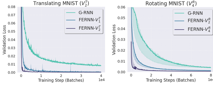
Figure 3: Increased flow equivariance increases training speed on data with flow symmetry. Validation loss vs. train steps.
