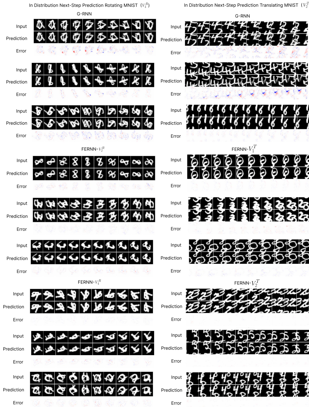
Figure 12: In-distribution sequence predictions for the models from Table 1 & Figure 3, trained on Rotating MNIST V_4^R (left) and Translating MNIST V_2^T (right), evaluated on the same flows.
