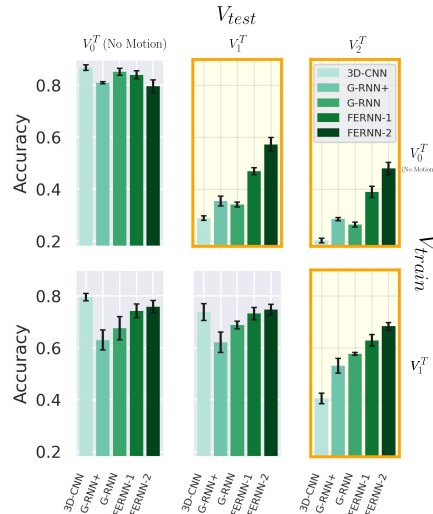
Figure 8: FERNNs outperform non-equivariant models on action recognition undergoing out-of-distribution flows (orange). Test accuracy of models trained on KTH with no motion V_0^T (top row) and with motion V_1^T (bottom row); tested on V_0^T , V_1^T , V_2^T (columns).
