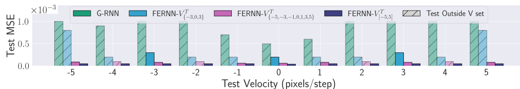
Figure 6: FERNNs can interpolate between \nu \in V . Test MSE for FERNNs trained and tested on x -translation velocity flows from -5 to +5 , with varying V -set coverage (see legend). Hatched bars indicate the test velocity is outside the model's equivariant set.
