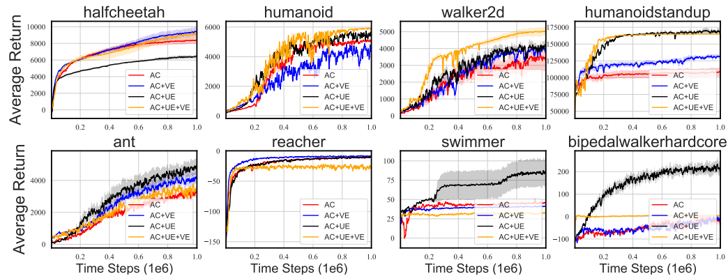
Figure 7: Learning curves of AC , AC+VE (SAC), AC+UE (DAC) and AC+UE+VE (DSAC) over five seeds across eight MuJoCo environments where DAC and DSAC are based on IQN. (First Row): Mutual improvement. (Second Row): Potential interference.
