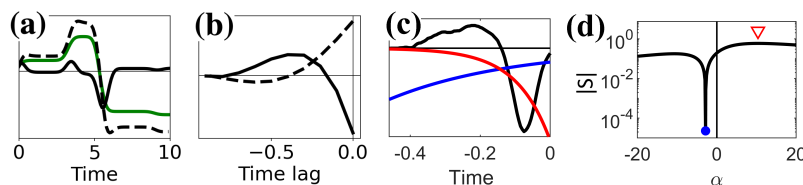
Figure 2: Data-driven temporal filters learned on the scalar time series from the natural image model compared with that of a bipolar cell. (a) Stimulus produced by the "dead leaves" model of natural images [53] (green), stimulus filtered through first (dashed black) and second (solid black) right singular vectors. (b) First (dashed) and second (solid) right singular vectors from Eq. (24) corresponding to predictive neurons. (c) Black: experimentally measured flash response of the salamander retinal bipolar cell (D.B. Kastner & S.A. Baccus, personal communication) on the inverted time axis approximates its linear filter. Compare this with the second singular vector (solid) in b. Note that the decay of the filter at zero time delay (absent in the theoretical result without additional constraints) is a consequence of causality and continuity of the filter implementation by a biological system. The maximally aligned (red) and the orthogonal (blue) exponentials are overlaid. (d) Cosine similarities of the temporal filters with a battery of exponentials. Blue dot indicates orthogonality and red triangle indicates maximum alignment. Closer alignment with expanding exponentials and orthogonality to a contracting exponential indicates the neuron's predictive nature.
