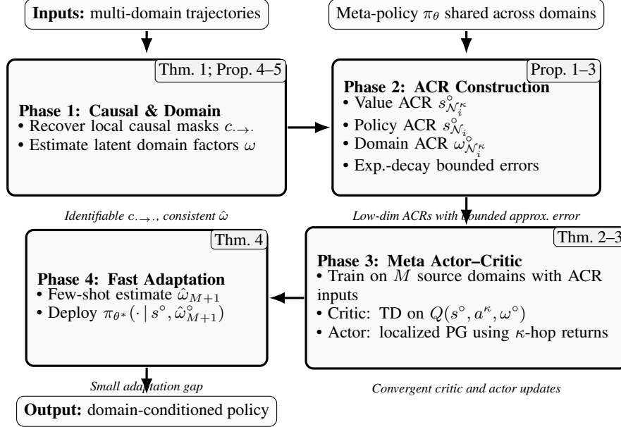
Figure 3: GSAC pipeline (cf. Algorithm 1). Each phase is annotated with its supporting results.
