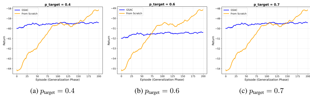
Figure 9: Adaptation comparison for different target domains in traffic control benchmark..
