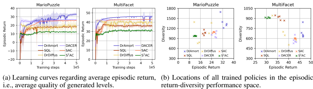
Figure 7: Evaluation results in the game content generation benchmark.
