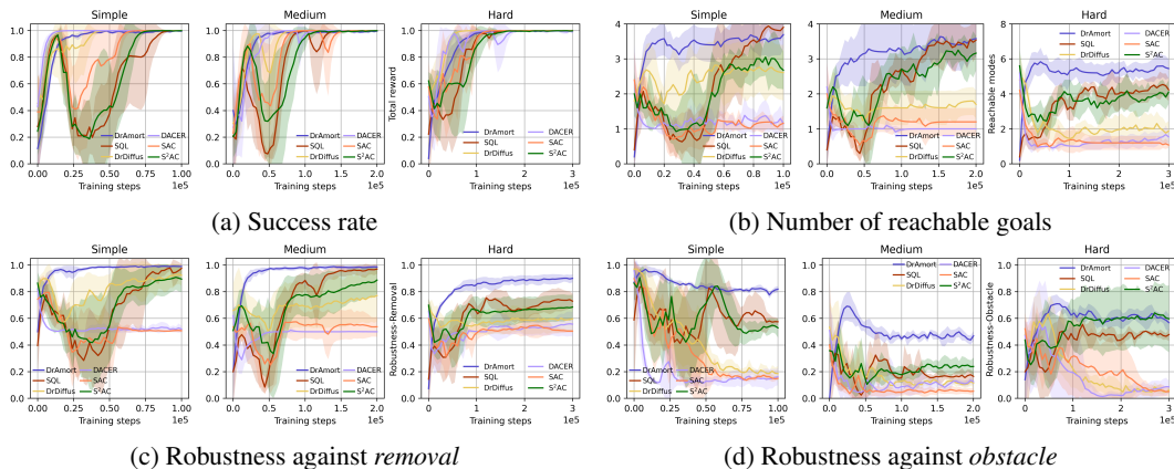
Figure 5: Learning curves in multi-goal PointMaze. Solid lines represent mean performance, and shaded regions indicate standard deviation. All curves are smoothed by the exponential moving average with a coefficient of 0.5.
