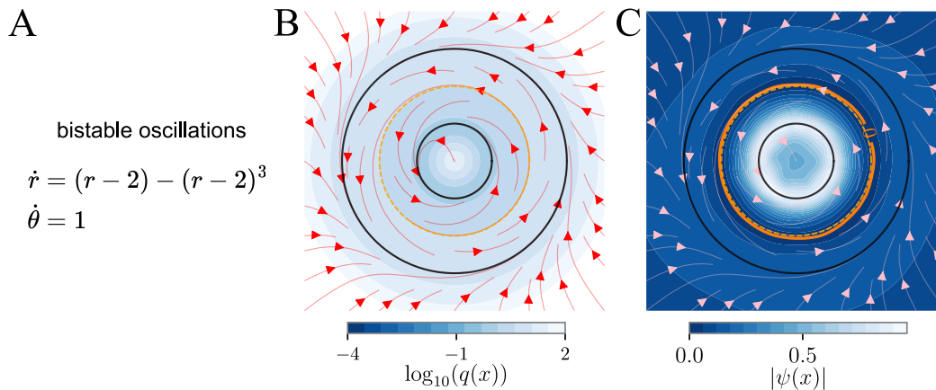
Figure 7: Applying our method to a system of stable and unstable limit cycles, a system without any fixed points on the separatrix. (A) system equations. (B) kinetic energy, with dashed line for separatrix. (C) KEF from our method with zero level highlighted.
