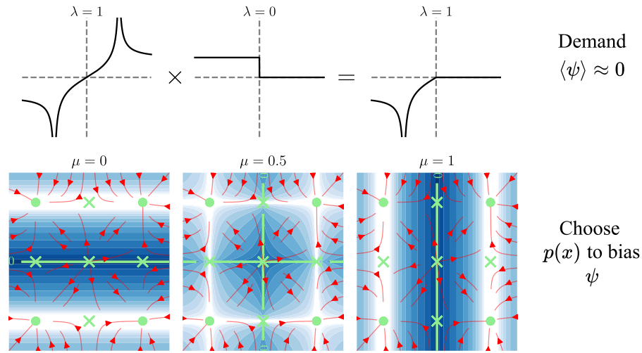
Figure 4: Top: In the presence of multiple basins, a KEF can collapse to zero within a single basin. This degeneracy is realised by multiplying the KEF with a piecewise constant KEF with \lambda = 0 and invoking (9). This example corresponds to \dot{x} = x - x^3 . We introduce a regularisation term (10) to encourage the mean value \langle \psi \rangle \approx 0 . This encourages solutions with sign changes across basins. Bottom: In higher dimensions, degeneracy arises from directional ambiguity in solutions. We visualise the analytical solution (12) for \dot{x} = x - x^3 ; \dot{y} = y - y^3 . We address this by sampling from multiple local distributions around separatrix points and training an ensemble of KEFs.
