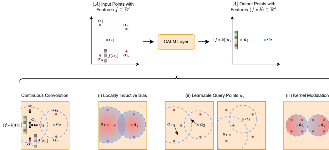
Figure 7: A CALM layer takes a point cloud with |\mathcal{A}| points as input and outputs a new point cloud with |\mathcal{A}| points and a new feature dimension d . CALM layers compute continuous convolution with a locality inductive bias to emphasize closer points, learnable query points (output positions), and a kernel modulation to allow different weights for different query points with similar translation vectors.
