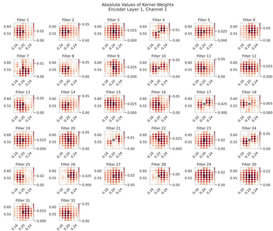
Figure 13: Absolute values of the kernel weights for the first layer of CALM-PDE's encoder trained on 2D Navier-Stokes. The black cross (x) represents the query point.
