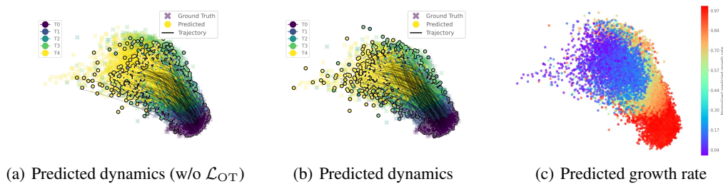
Figure 4: Visualization of predicted dynamics by (a) VFGM (w/o \mathcal{L}_{OT} ) and (b) VGFM, and growth rate by (c) VFGM, on EB (5D) dataset, where the hold-out time is the first intermediate timepoint.
