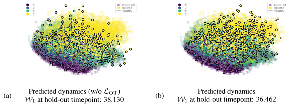
Figure A-14: Visualization of predicted dynamics by (a) VFGM (w/o \mathcal{L}_{OT} ) and (b) VFGM on CITE (50D) dataset, where the hold-out time is the second intermediate timepoint.
