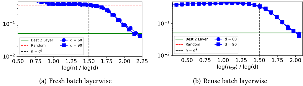
Figure 6: Reuse of the same data batch over layers: The plots compare the generalization error achieved by two variants of the layerwise procedure in Theorem 1. The left panel illustrates a routine without using the same batch of data for different layers of training, while on the right this assumption is relaxed by always holding constant the total number of samples seen for every layer. There is no substantial difference between the two algorithms when looking at the generalization performance. The target is f^*(\mathbf{x}) = \tanh\left(\mathbf{a}^{*\top} P_3(W^*\mathbf{x})/\sqrt{d^{\varepsilon_1=1/2}}\right) and the hyperparameters are listed in Sec. F.4.
