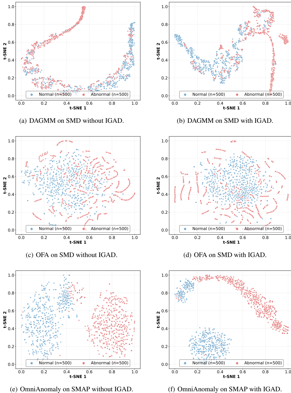
Figure 11: The visualization of latent space using t-SNE before and after applying IGAD.
