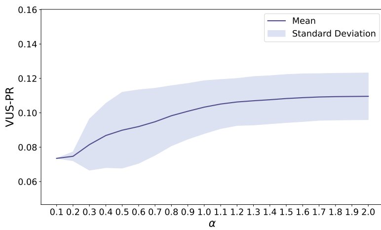
(c) \alpha
