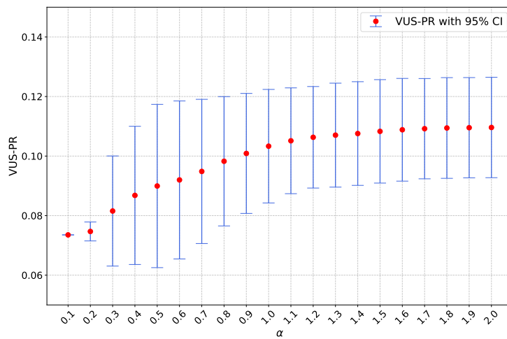
(c) \alpha
