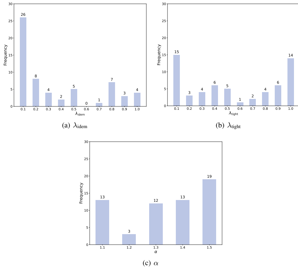
Figure 8: Parameter frequency records for \lambda_{\text{idem}} , \lambda_{\text{tight}} and \alpha .
