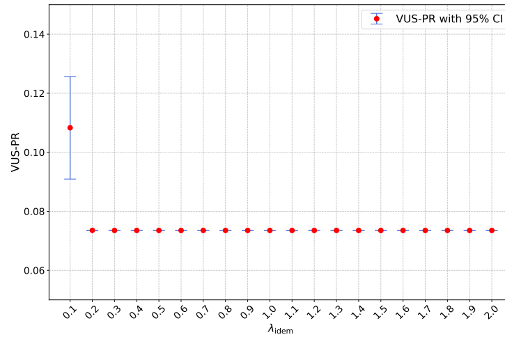
(a) \lambda_{idem}
