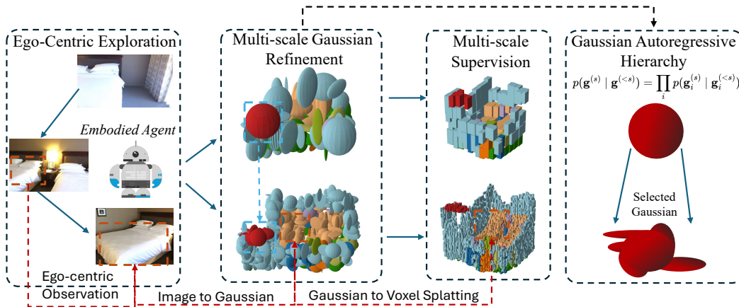
Figure 1: Overview of the proposed DF Gauss framework. An embodied agent acquires egocentric RGB observations while navigating the environment, which are transformed into multi-scale Gaussian representations for autoregressive refinement. A selective masking strategy focuses computation on informative regions. In the illustrated example, the model identifies a bed (shown in peach) and ceiling (shown in dark red) through hierarchical Gaussian updates.
