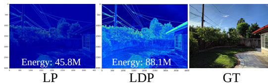
Figure 2: Example of high-frequency information extracted from the Laplacian pyramid (LP) and our LDP. We can observe that our LDP extracts high-frequency information more effectively than LP.
