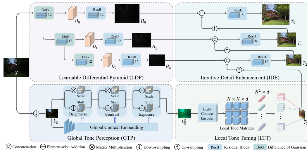
Figure 3: The overall pipeline of our DPRNet. It includes the proposed Learnable Differential Pyramid (LDP), Iterative Detail Enhancement (IDE), Global Tone Perception (GTP), and Local Tone Tuning (LTT). The LDP, in synergy with the IDE, is responsible for extracting and enhancing the high-frequency details. The GTP collaborates with LTT to achieve globally consistent yet locally fine-grained tone mapping.
