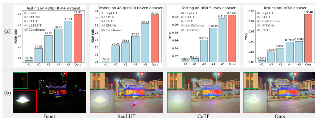
Figure 1: (a) Our DPRNet provides remarkable performance gains on the four datasets. (b) Existing tone mapping methods suffer from detail loss and halo artifacts.
