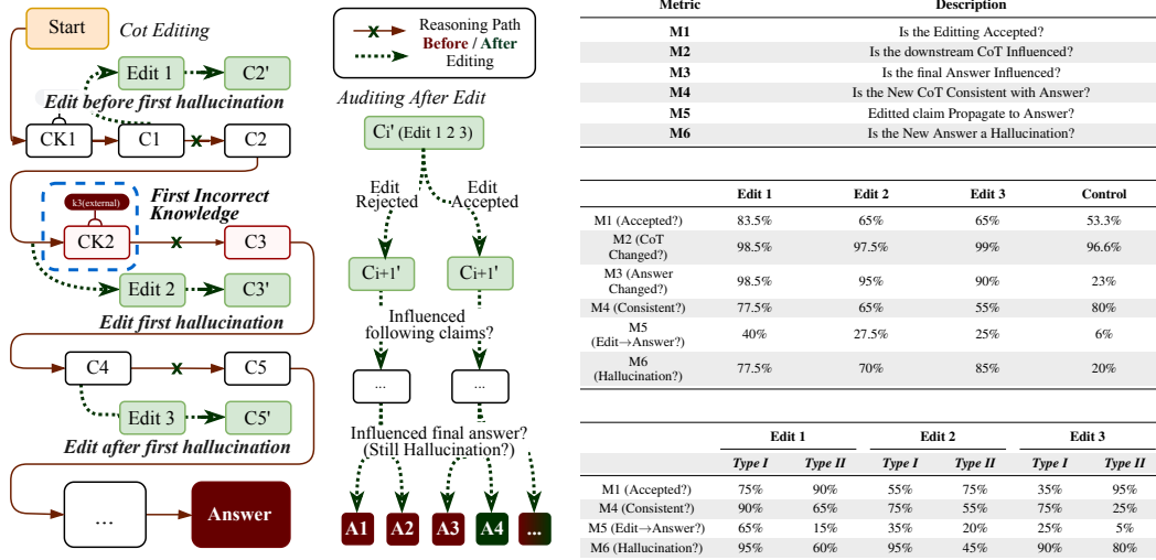
Figure 3: Design and results of our CoT editing experiments. (1) The left diagram illustrates the process of modifying CoT, where edits are introduced at three distinct intervention edit points. (2) The right tables present the corresponding evaluation results. Top: metric indices and their descriptions. Middle: comparative statistics across different edit points for hallucinated cases and their respective controls. Bottom: Type-wise breakdown across Type I and Type II hallucinations.
