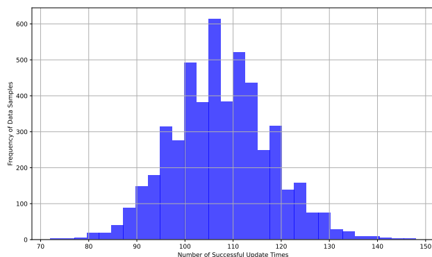
Figure 7: Distribution of data samples' successful update: Histogram of all training data samples' successful update. The average count is 107.53 (\pm 10.27) and the min and max are 72 and 148, respectively.
