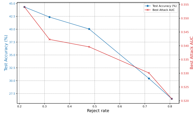
Figure 5: Privacy-utility trade-off with fixed Reject rate: We show the privacy utility trade-off with fixed reject rate by using adaptive \gamma during training. We can observe that with a higher reject rate, defense performance is improved, but utility is lower.
