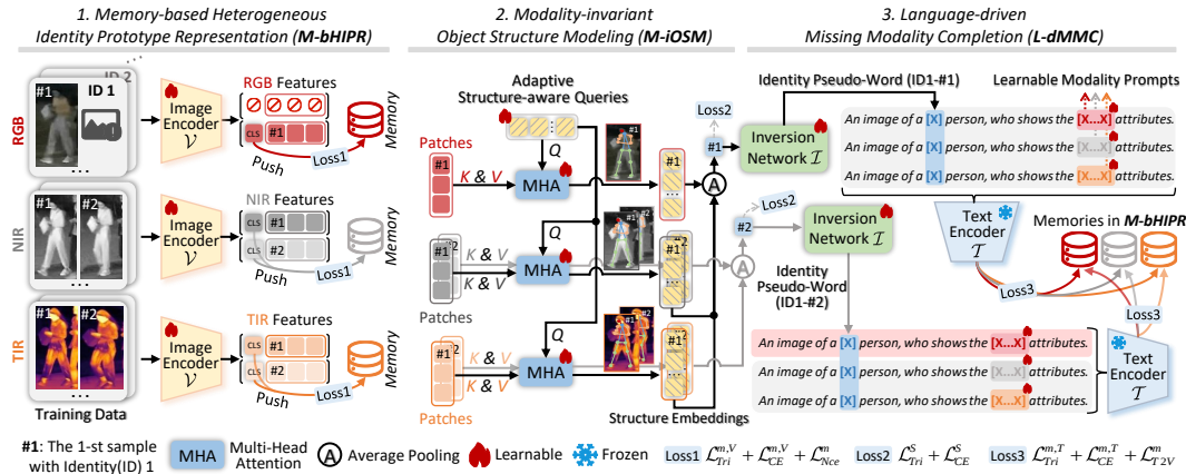
Figure 2: Pipeline of the proposed Miss-ReID under modality-missing training conditions.
