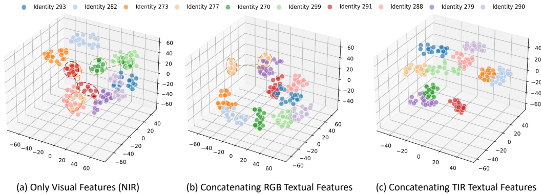
Figure 6: The feature distributions of 10 identities randomly sampled from the RGBNT201 dataset by using t-SNE [41]. Here, we take the challenging case ( RNT ) that both RGB and TIR images are unavailable as an example. (a) The vision-only features derived from available NIR images. (b) The fused features that concatenating the compensatory RGB textual features on (a). (c) The fused features that further concatenating the compensatory TIR textual features on (b). Different colors refer to different identities.
