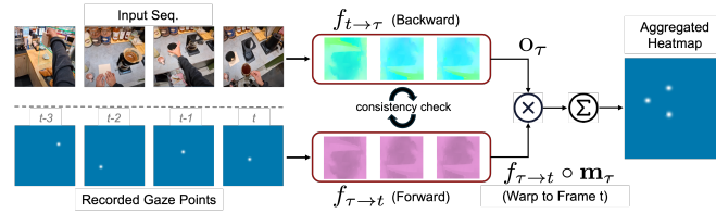
Figure 2: Temporal Aggregation of Gaze. Top: Input egocentric frames. Bottom: Gaze points transformed into heatmaps, filtered using bidirectional optical flow ( f_{\tau \rightarrow t} , f_{t \rightarrow \tau} ) to remove occluded points, then warped and aggregated into a temporally coherent supervision signal.
