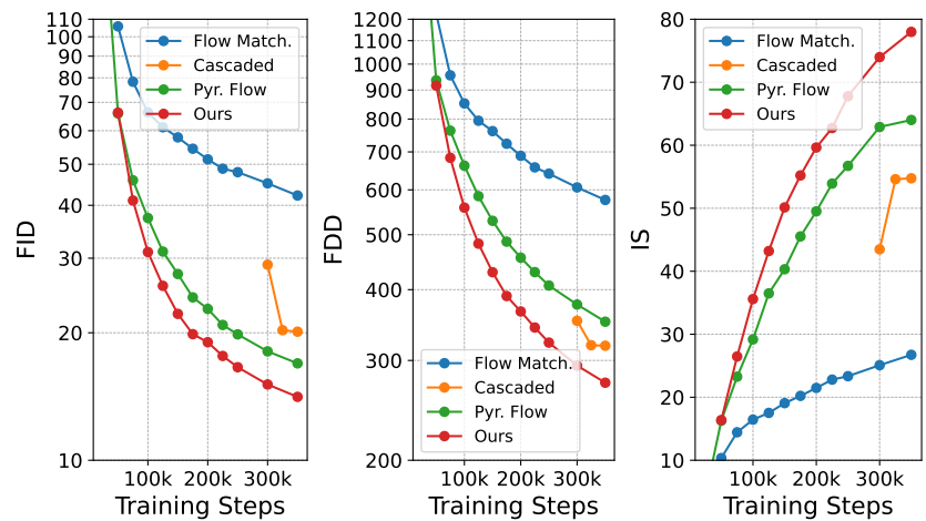
Figure 9: Convergence curves for different datasets and metrics comparing our framework to baselines on ImageNet-1K [5] 1024px.
