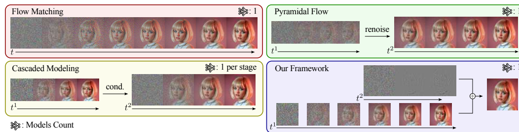
Figure 1: Comparison of different diffusion frameworks. Cascaded models employ a separate model per stage. Pyramidal Flow [18] progressively increases resolution through careful upsampling and renoising operations. Our framework models multiple stages independently from each other within the same model, enabling progressive generation with minimal modifications to Flow Matching [27]
