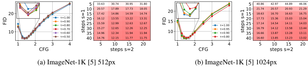
Figure 3: FID 10K results ablating sampling configuration, threshold, and per-stage steps.
