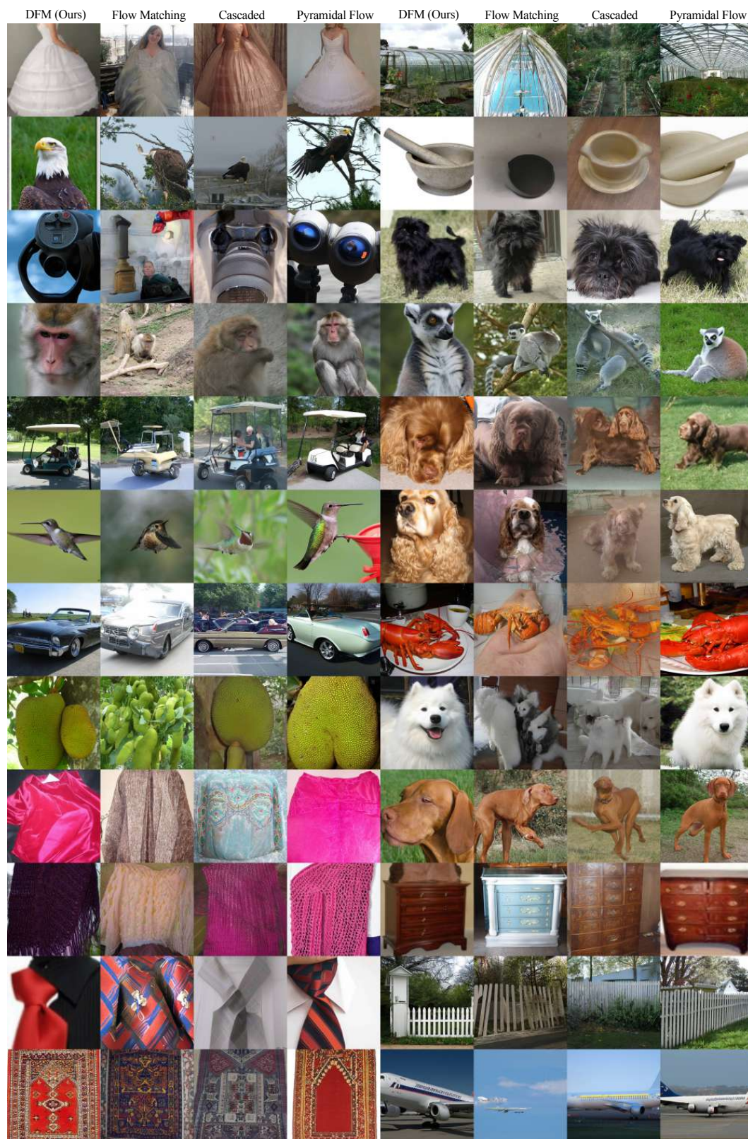
Figure 12: Comparison of DFM against baselines on DiT-XL trained on ImageNet-1K 1024px [5] for 350k steps. Samples are fully uncensored and generated with cfg 3.0.
