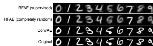
Figure 8: MNIST digit reconstructions produced by RFAE using supervised and completely random forests, and by a convolutional autoencoder; original images are displayed in the bottom row.
