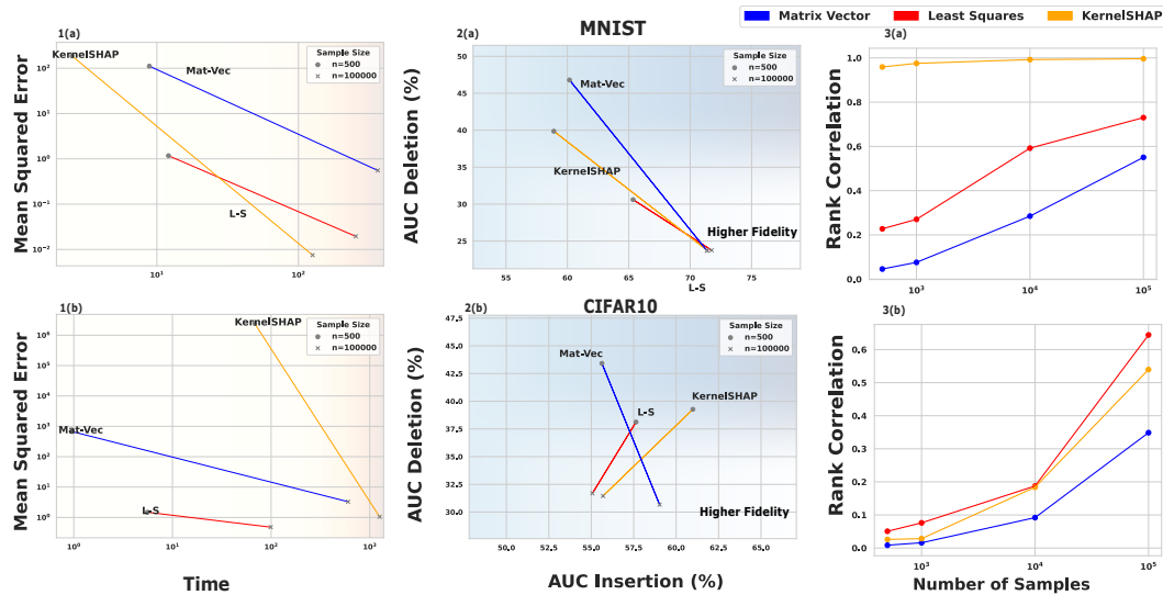
Figure 3: Comparison of estimators in image datasets: MNIST (top row) and CIFAR (bottom row). In the first column, (1, left column) performance of estimators is measured with mean squared error (normalized) from true Shapley value and time (in seconds). (2, center column) Area under the curve (AUC) calculation for insertion (x-axis) and deletion curves (y-axis) have been provided, computed on the top 100 features; reported as percentage under the curve. (3, right column) Spearman rank correlation for increasing number of samples.
