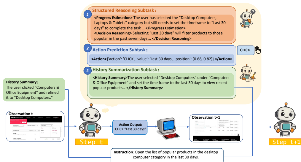
Figure 1: GUI-Rise agent framework overview. It introduces a three-subtask framework that integrates structured reasoning, action prediction, and history summarization. At each step, the agent performs structured reasoning (progress estimation and decision analysis), predicts the next GUI action, and updates a compact history summary for the next iteration.
