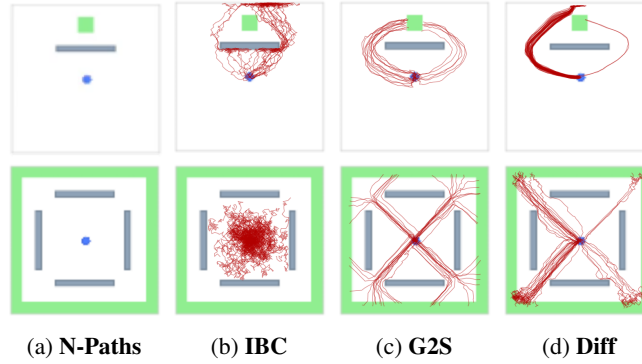
Figure 8: Multimodal Behavior. From the start state (blue) there are two paths (top row) and four paths (bottom row) to the goal state (green). When using high enough angular frequency ( L = 2 , L = 4 ), G2Sphere learns all paths and commits to a path at the start of each rollout. Diffusion Policy exhibits a similar behavior but shows some bias towards certain paths whereas IBC fails to learn due to an equal distribution of expert path data.
