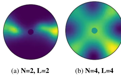
Figure 9: Energy Landscape. We visualize the energy landscapes generated with the G2Sphere on the N-Paths domain with N = 2 and N = 4 , respectively.
