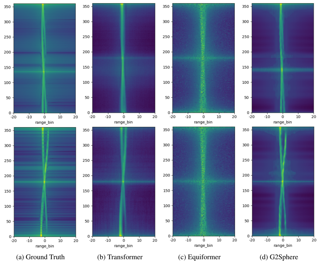
Figure 14: Frusta Radar Predictions. Radar response predictions on the Frusta dataset. Due to the roll symmetry in the Frusta dataset we plot the spherical outputs as static patterns. G2Sphere is best able to capture both the overall structure of the response and also the speculars (bright horizontal lines).
