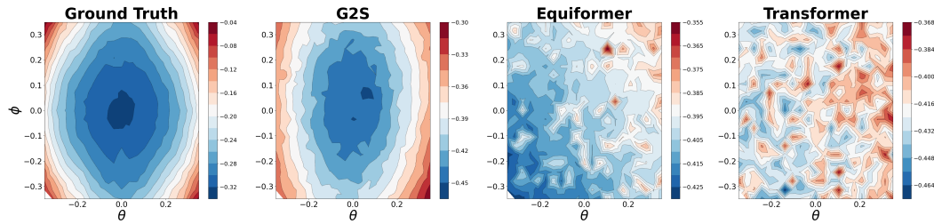
Figure 4: Generalizing to Unseen Objects. Full drag prediction on test sample not included in the Pods dataset. Unlike in our training dataset, we compute the entire drag prediction from -20 to 20 degrees (shown in radians here). Despite being trained on single coordinate points, G2Sphere is able to reconstruct the general shape of the drag function, whereas the baseline implicit models overfit to specific points.
