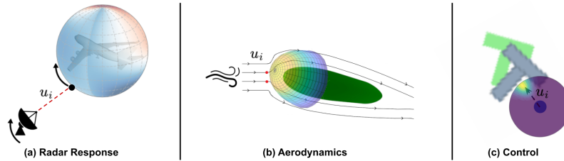
Figure 1: Spherical Domains. Across many different domains learning high-frequency spherical signals is a challenging task. (a) In the radar response domain, we learn a function F_X(u_i) , which maps the input geometry X and the radar viewing angle u_i to the radar response. (b) In the aerodynamics domain, we learn a function F_X(u_i) , which maps the input geometry X and the airflow direction u_i to the corresponding drag coefficient. (c) In the control domain, we learn a function F_X(u_i) , which maps the environmental geometry X and the control action u_i to their value.
