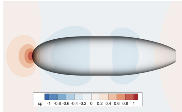
Figure 12: Aerodynamics Simulator. Ground truth drag coefficients generated by the numerical CDF simulator.
