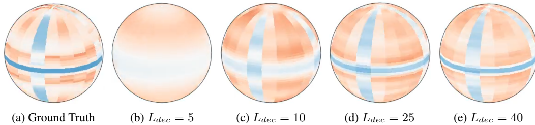
Figure 6: Effect of L_{dec} on Fidelity. As the maximum frequency of the decoder increases so does the accuracy of the G2Sphere prediction. At L_{dec} = 5 we see that most of the features of the signal are lost and we are only capable of modelling the general high/low signals. However, as we increase to L_{dec} > 5 we can see the features getting sharper as the output frequency increases.
