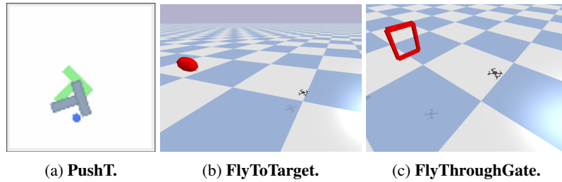
Figure 13: Policy Learning Domains. The tasks from our policy learning benchmarks. The fixed-goal variant of PushT is shown in (a). The target position to fly to is shown as a red ball in (b) and the gate to fly through is shown in red in (c).
