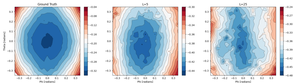
Figure 7: Effect of L_{dec} on Generalization. As the maximum frequency of the decoder increases, G2Sphere starts to overfit to the sparse data samples in the Drag domain. As a result, the G2Sphere model with a lower output frequency generalizes better to new data.
