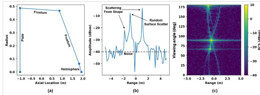
Figure 11: Radar Simulator. (a) Cross section of random 3D object mesh. (b) The range profile for 20^\circ viewing angle. (c) The corresponding static radar pattern.
