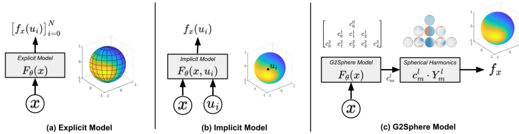
Figure 5: Modeling Spherical Functions. (a) The explicit model outputs a fixed grid of predictions to approximate the continuous function f_x . (b) The implicit model learns f_x by conditioning on both input x and coordinate point u . (c) G2Sphere decomposes f_x into a set of learned Fourier coefficients c_l^m and spherical harmonics Y_l^m . This enables prediction of f_x at any coordinate point u .
