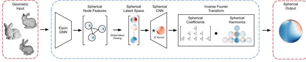
Figure 2: G2Sphere Architecture. Illustration of the G2Sphere (G2S) model. First, the geometric input is converted from real space (red dotted-line) to Fourier space (blue dotted line) using an SO(3) -equivariant encoder. We decode this spherical latent representation into a set of Fourier coefficients c_m^l representing the continuous spherical signal. Finally, these coefficients are combined with a grid of pre-computed harmonic basis functions to convert back to real space.
