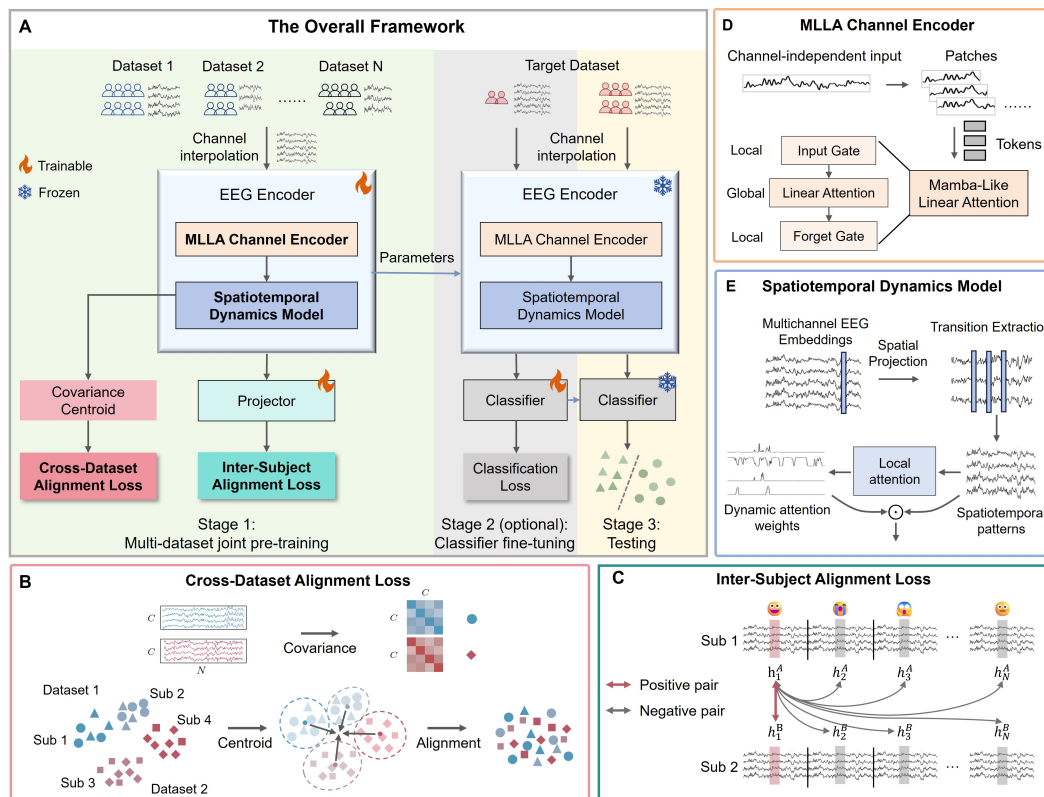
Figure 2: The overall framework, model architectures, and loss designs of mdJPT. A) The overall framework. Our approach comprises three stages: multi-dataset pre-training, optional classifier fine-tuning, and testing. The EEG encoder integrates an MLLA channel encoder with a spatiotemporal dynamics model. Pre-training combines CDA and inter-subject alignment (ISA) losses. The resulting model supports either zero-shot generalization or fine-tuning with a lightweight classifier on limited target data. Final evaluation is performed on held-out subjects. B) The cross-dataset alignment loss. The covariance is calculated from the latent representations, and covariance centroids of subjects from different datasets are aligned. C) The inter-subject alignment loss. EEG samples from two subjects corresponding to the same time segment within a trial are regarded as positive samples, and those corresponding to different trials are regarded as negative samples. A contrastive loss is employed to pull together the positive samples and push apart the negative samples. D) MLLA channel encoder. A channel-independent Mamba-like linear attention encoder is employed to process the time-slided patches of each EEG channel. E) Spatiotemporal dynamics model. The multichannel EEG embeddings are processed by spatial projections and transition extraction to obtain spatiotemporal EEG patterns, then a local attention is employed to estimate dynamic attention weights on these patterns.
