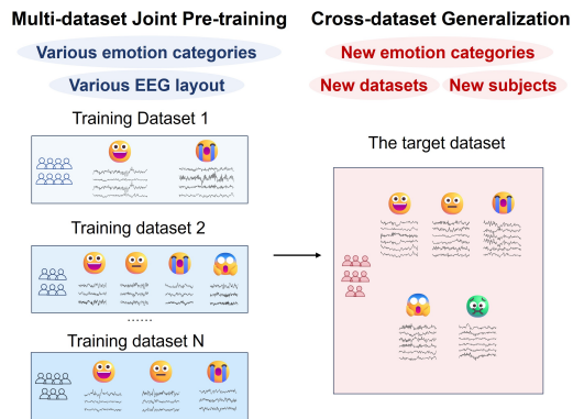
Figure 1: Cross-dataset generalization through multi-dataset pre-training. (left) Challenges of task-specific EEG pre-training. (right) Challenges of inference.
