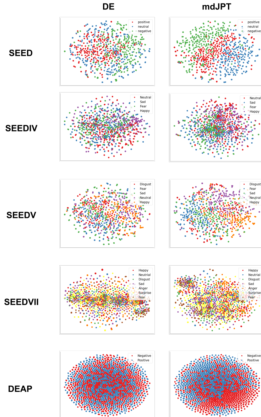
Figure S3: t-SNE visualization of extracted feature on SEED, SEED-IV, SEED-V, SEED-VII, and DEAP datasets. The EEG encoder used for feature extraction was trained on all datasets other than the target dataset.
