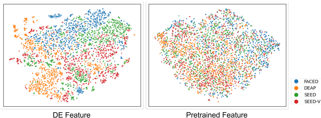
Figure 3: t-sne visualization of features. Compared to DE, pretrained features show better cross-dataset alignment, with features from different datasets more evenly intermixed.
