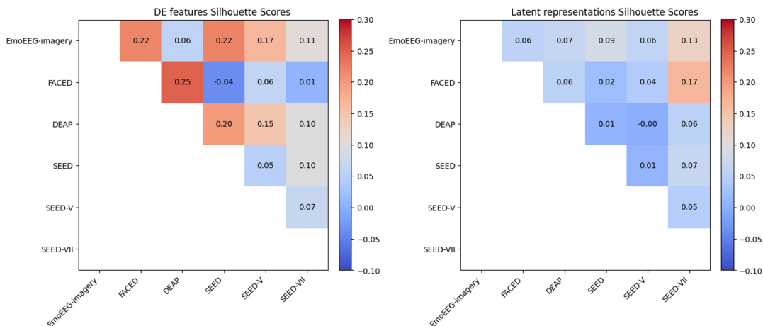
Figure S2: Average silhouette score between features of different datasets.
