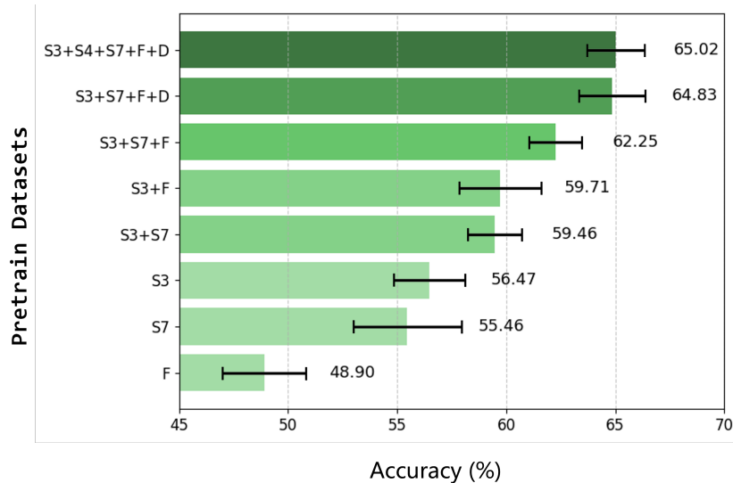
Figure 4: Generalization performance of mdJPT with an increasing number of datasets. Few-shot setting is used here with SEED-V dataset as the testing dataset. Abbr. S3, S4, S7, F, D stand for SEED, SEED-IV, SEED-VII, FACED, and DEAP, respectively.
