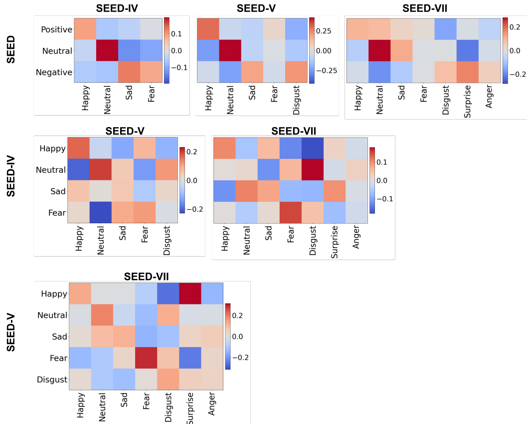
Figure S5: Pearson correlation coefficient between emotion-related feature importance weights on different datasets
