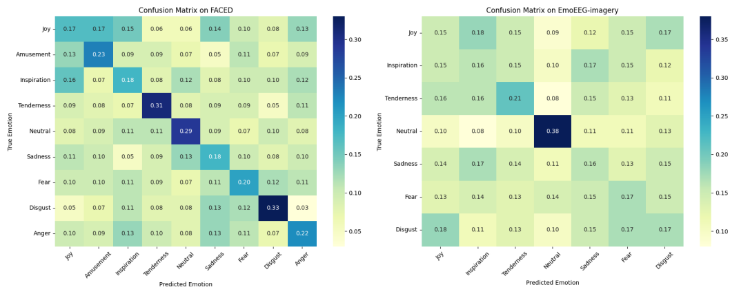
Figure S1: Confusion matrices of emotion classification results on FACED and EmoEEG-imagery datasets.
