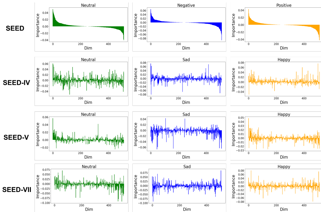
Figure S4: Comparison of feature importance attribution for neutral, negative/sad, and positive/happy emotions on SEED, SEED-IV, SEED-V, and SEED-VII datasets. The feature indices are sorted by the feature importance on the SEED dataset.
